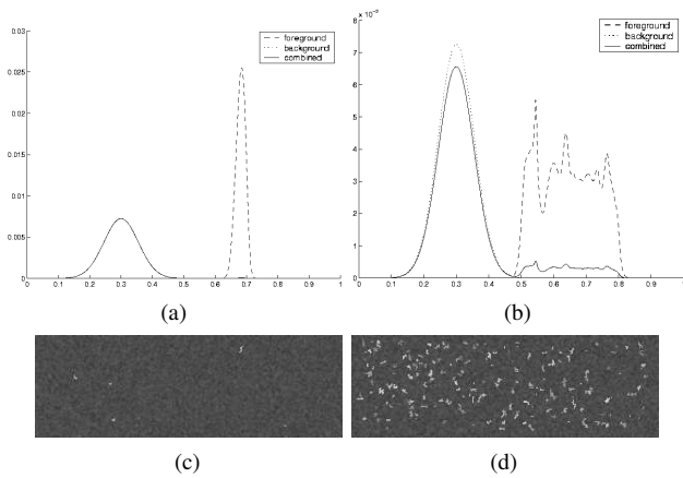
Figure 3: Model-generated histograms and the corresponding artificial images: (a),(c) Foreground/background ratio 0.001; (b),(d) 0.05.
