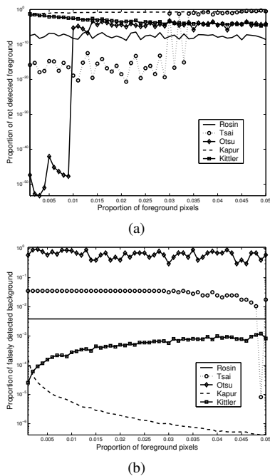
Figure 4: Detection results for artificial data: (a) proportion of not detected foreground pixels, and (b) proportion of falsely detected background pixels.
